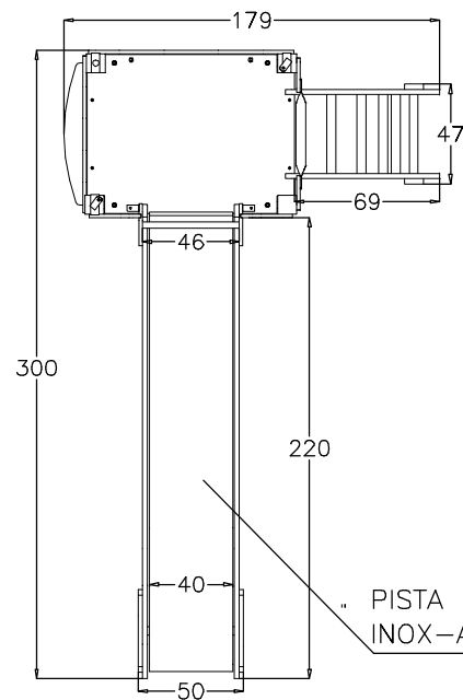
PIANTA (PLAN)
