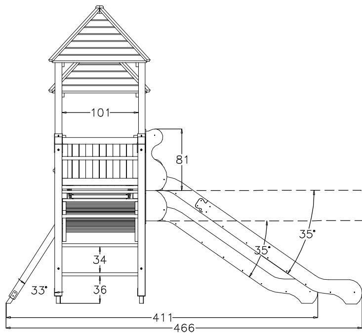
VISTA LATERALE (LATERAL VIEW)
