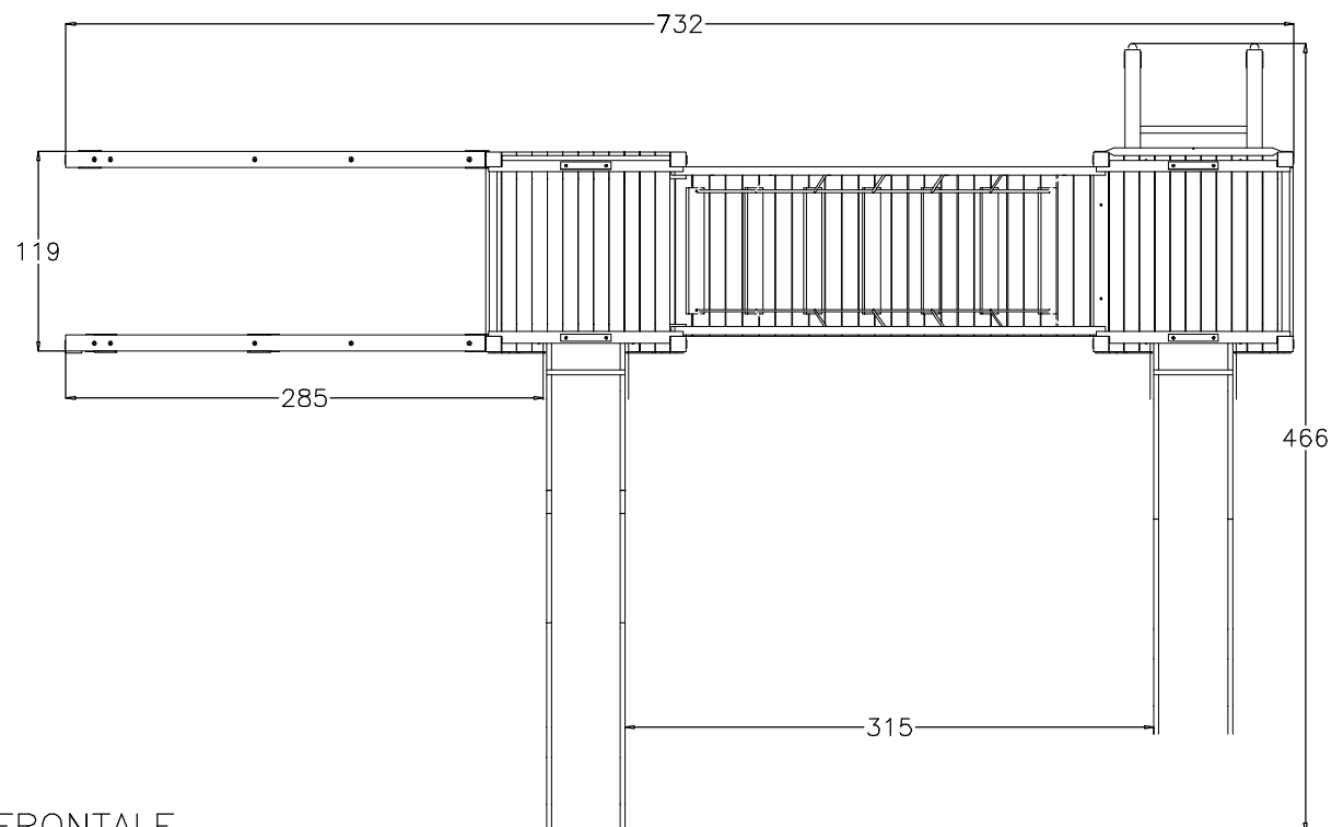
VISTA FRONTALE (FRONTAL VIEW)
