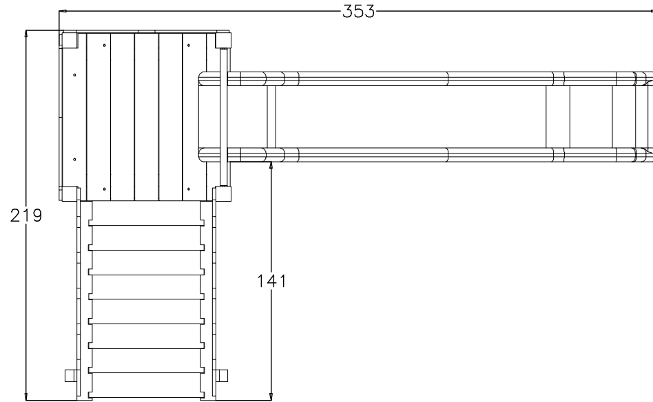
PIANTA (PLAN)
