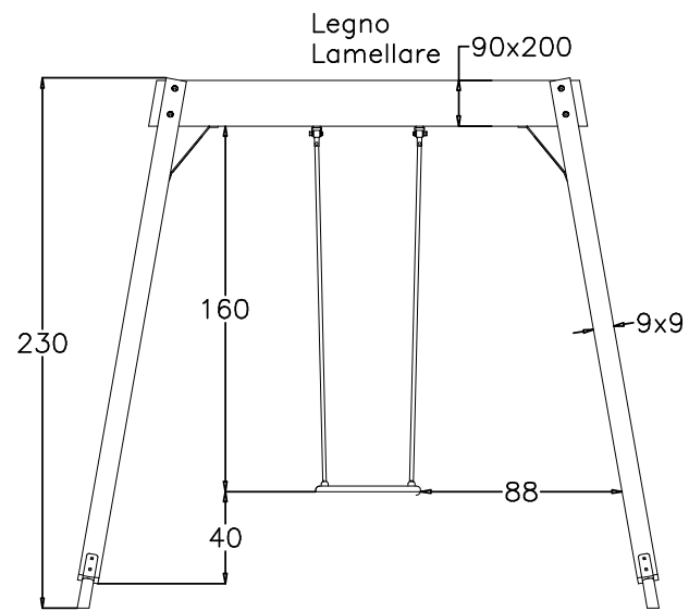
VISTA LATERALE (LATERAL VIEW)
