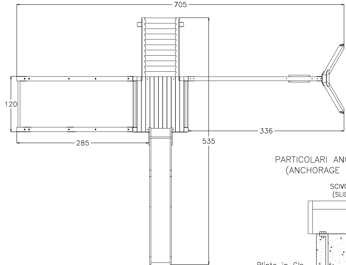
PIANTA (PLAN)
