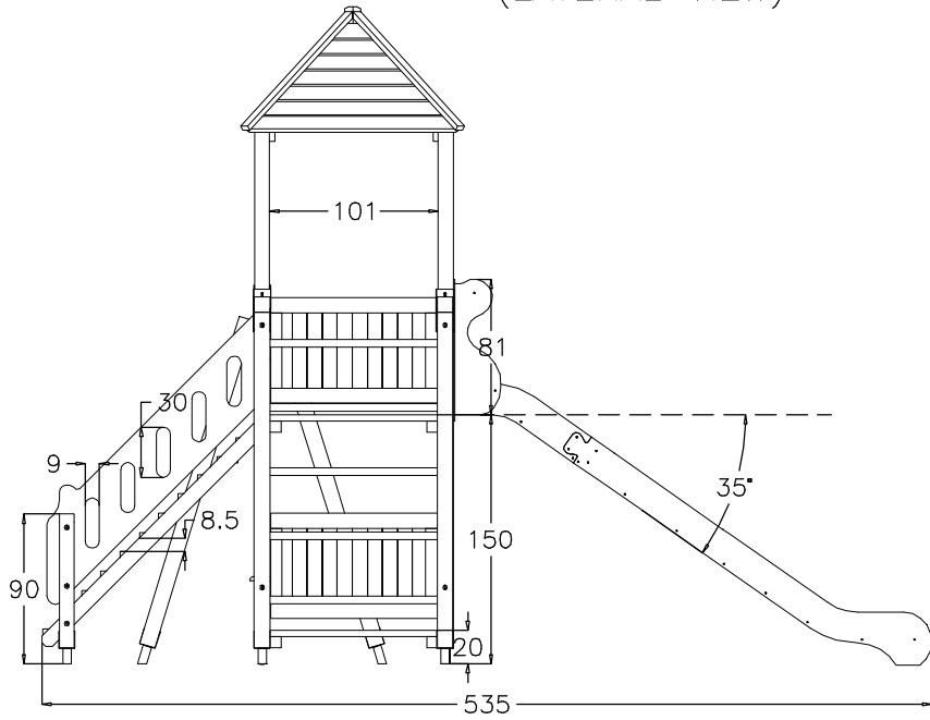
VISTA LATERALE (LATERAL VIEW)
