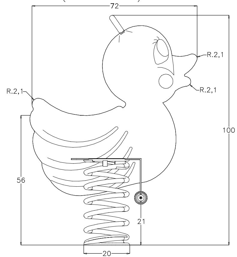
VISTA LATERALE (LATERAL VIEW)
