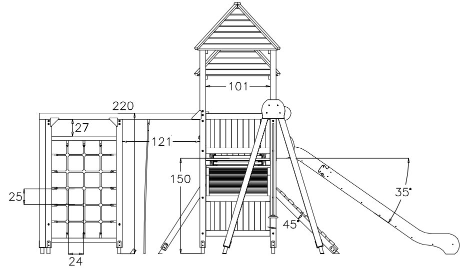
VISTA LATERALE (LATERAL VIEW)
