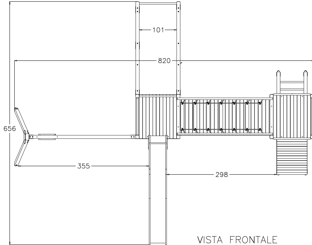
PIANTA (PLAN)
