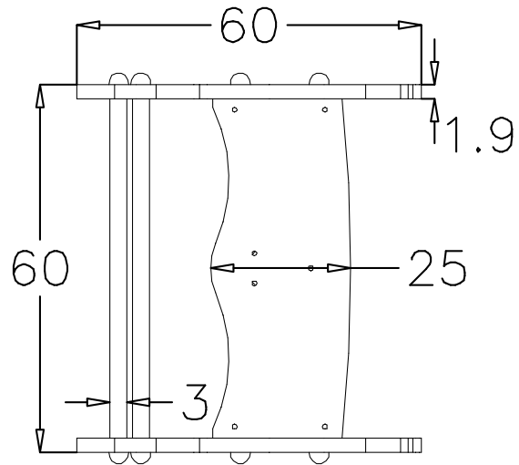
PIANTA (PLAN)
