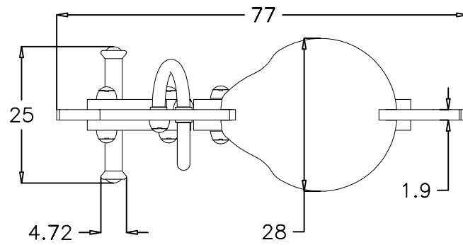
PIANTA (PLAN)
